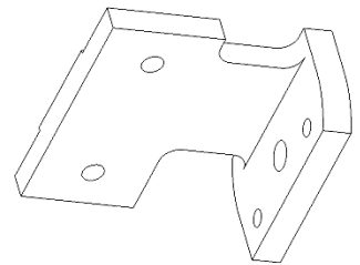
Figure 12 (A00280 & A00281)
