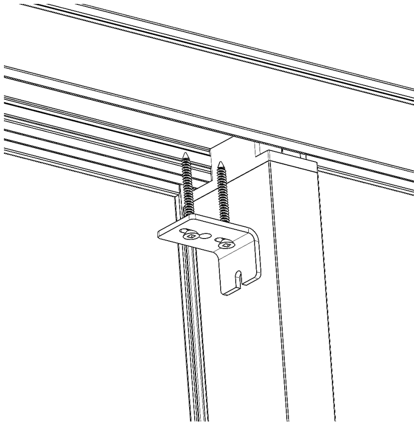
Figure 19 With panels in final positions, locate and install the corresponding head fillers into their respective head tracks.
