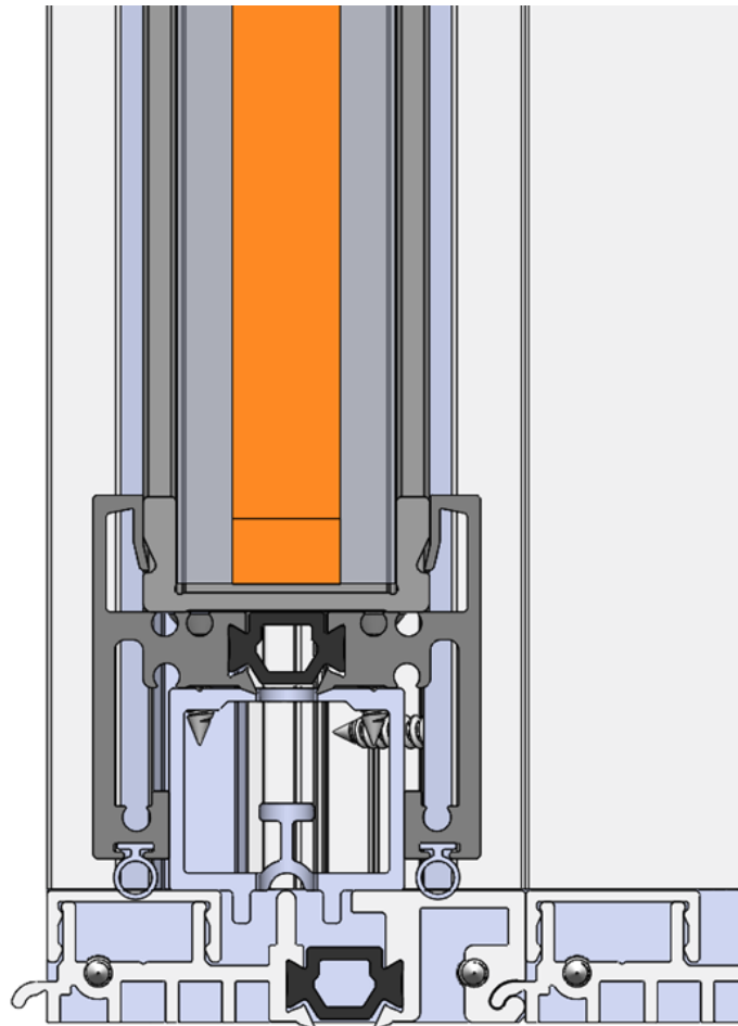
Section view through sill and bottom rail showing alignment of riser block.
