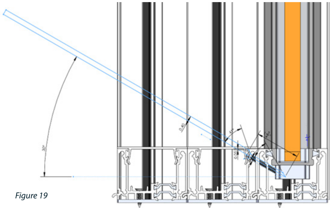
Section view through sill and bottom rail showing alignment of riser block.
