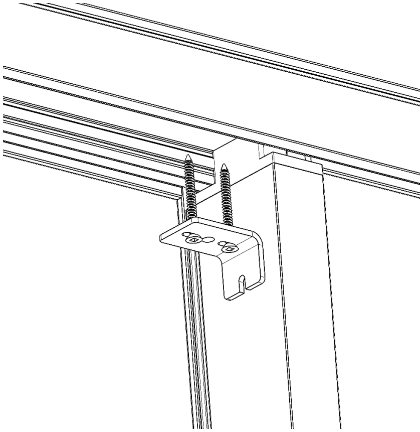
Figure 19 With panels in final positions, locate and install the corresponding head fillers into their respective head tracks.
